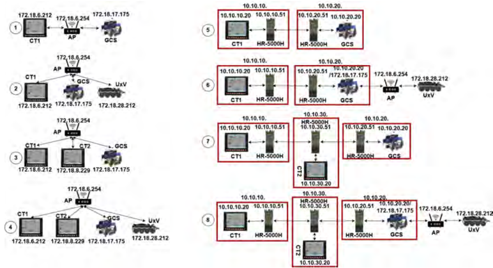
Figure 5.2: Connection Time, Key Renewal, System Reliability, Goodput Estimation and CPU Processing Time Testing Architecture.
