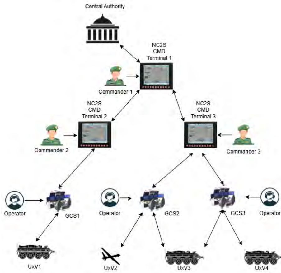
Figure 4.1: NC2S Architecture.
