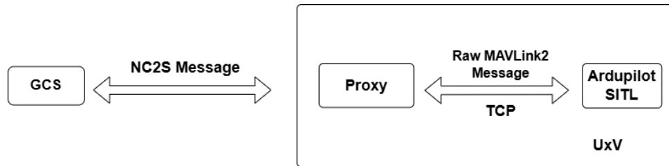
Figure 4.3: UxV Architecture.
