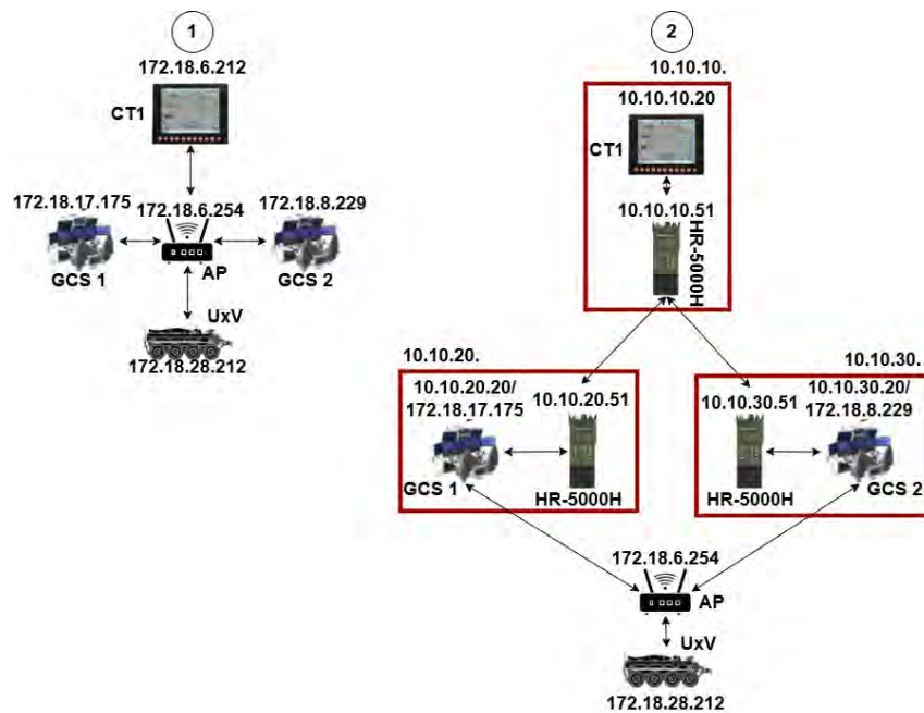
Figure 5.3: Handover Testing Architecture.
