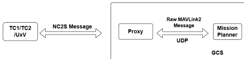
Figure 4.2: GCS Architecture.
