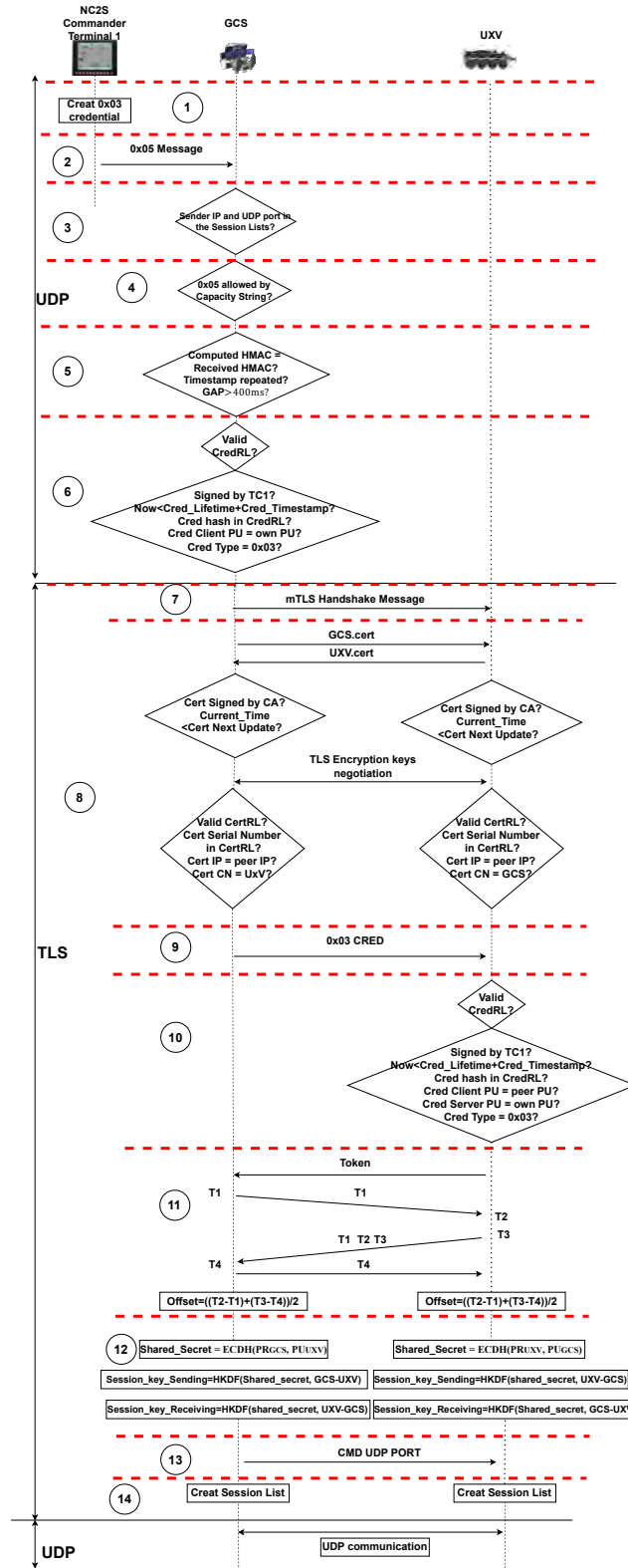
Figure A.4: TC1-GCS-UxV
