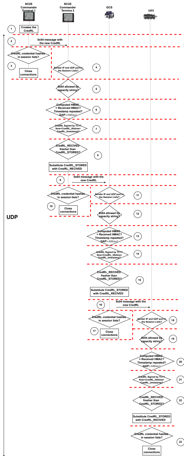
Figure A.6: Credential Revocation Protocol
