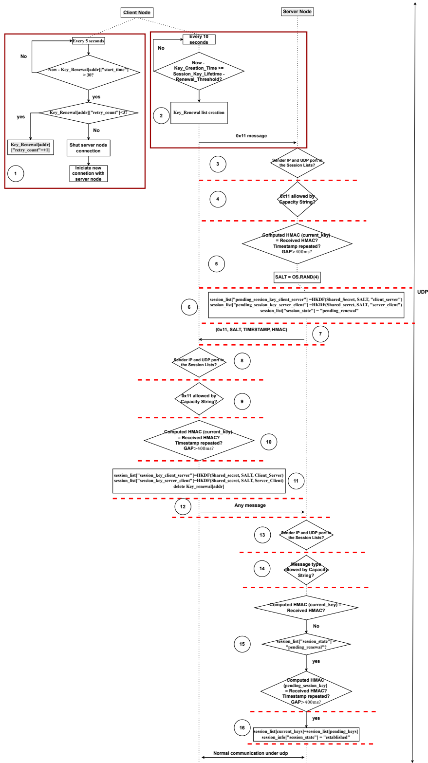
Figure A.9: Key Renewal Protocol
