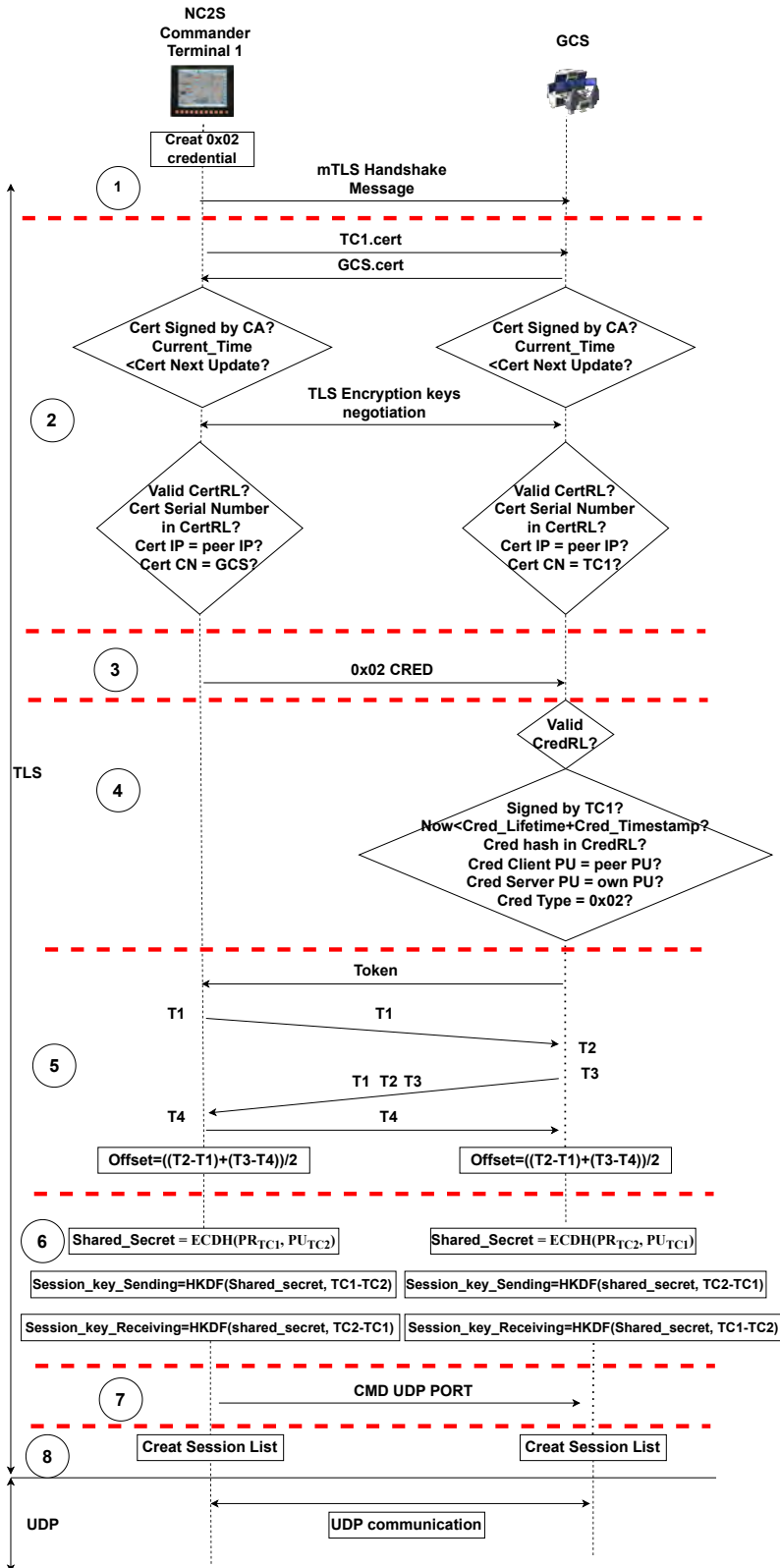
Figure A.1: TC1–GCS Connection Establishment
