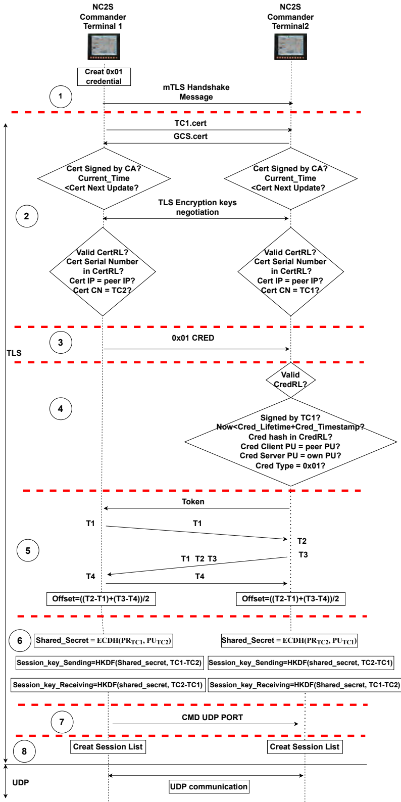
Figure A.2: TC1–TC2 Connection Establishment
