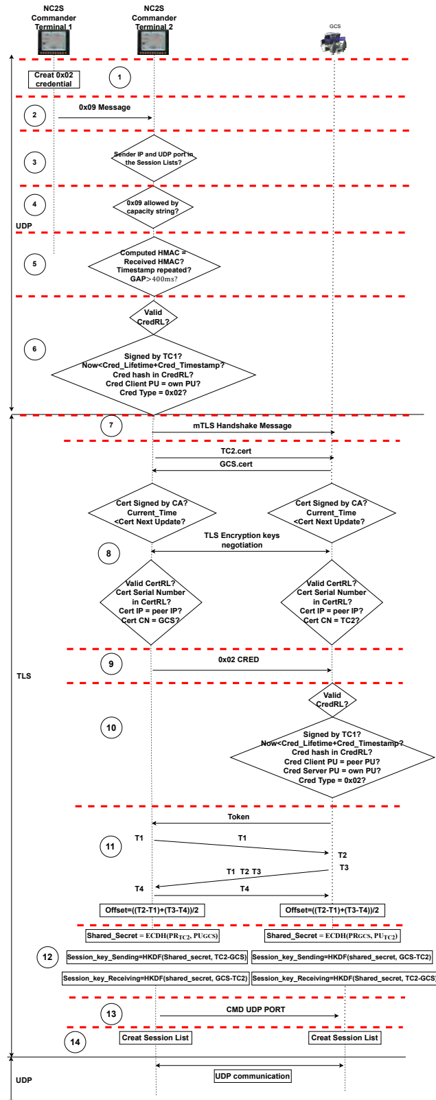
Figure A.3: TC1–TC2–GCS 91
